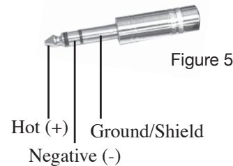
Balanced TRS 1/4" Plug
