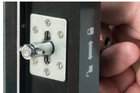
Note horizontal orientation of the locking-tab mechanism with the tab in locked position
